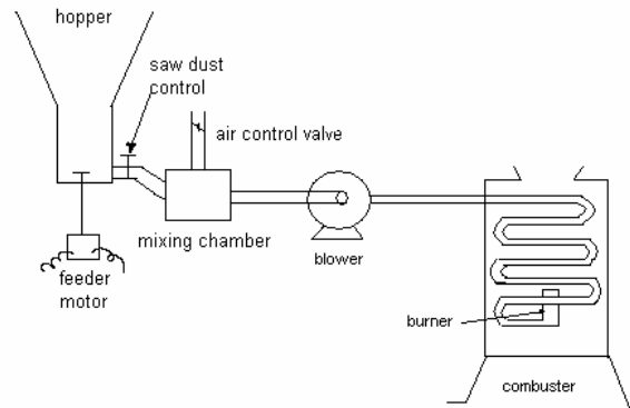
Figure 1: Schematic of the Sawdust Combustor with Accessories
